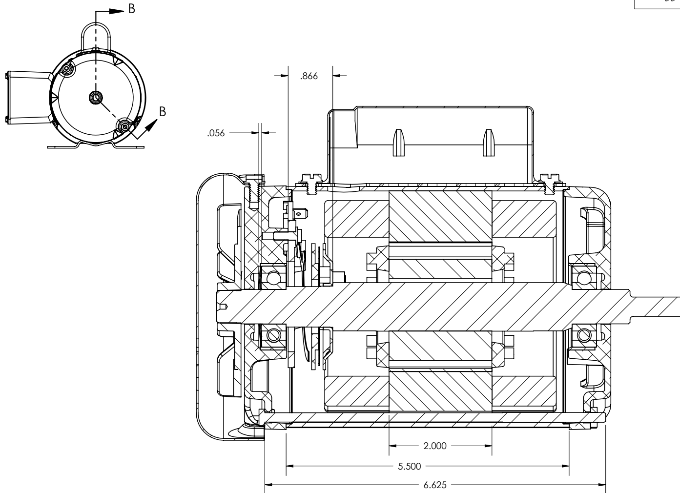
SECTION B-B
