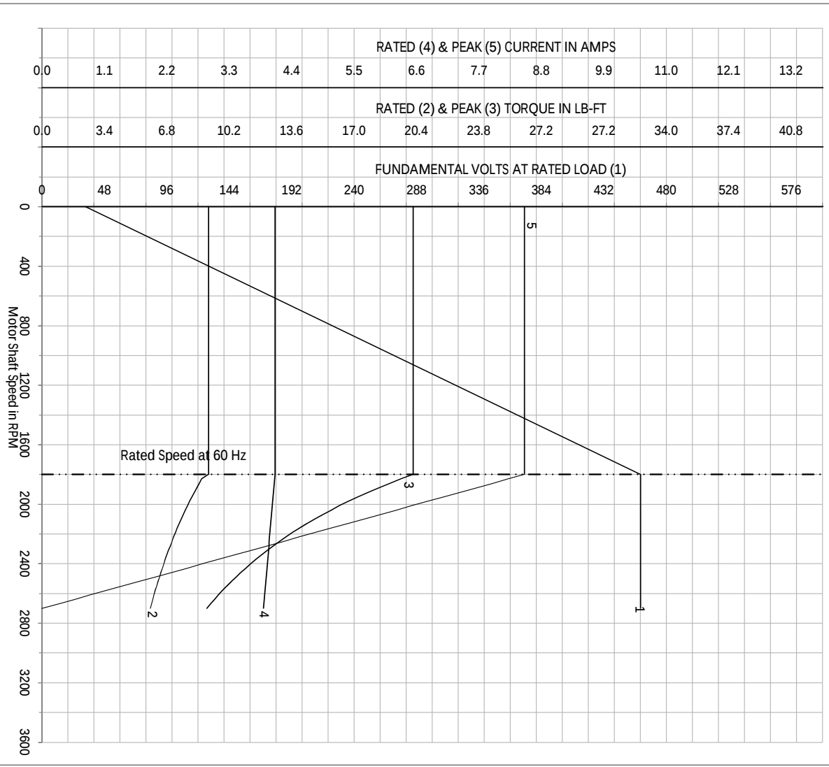
Variable Speed AC Motor Curves
