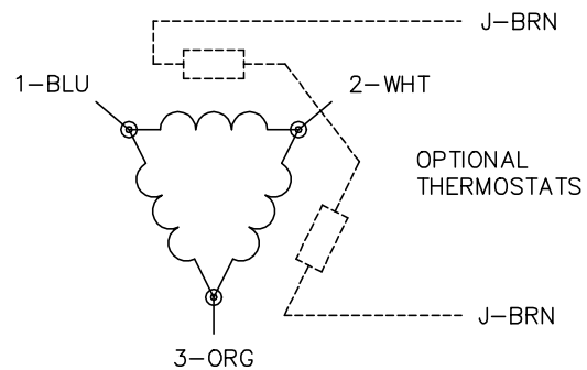
TYPICAL DELTA-CONNECTED MOTOR
