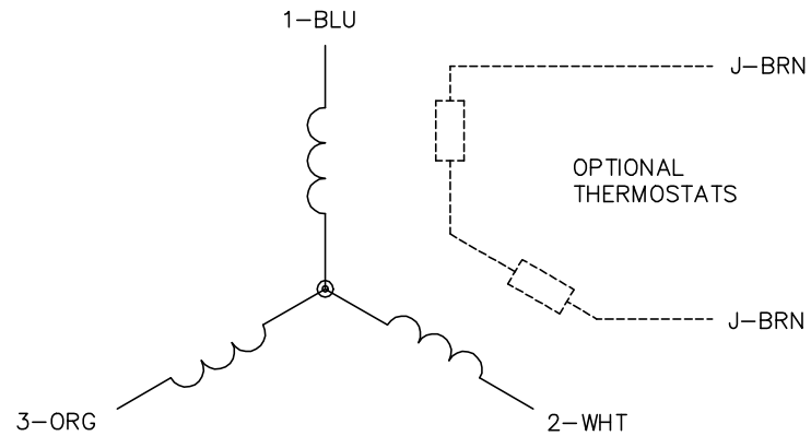
TYPICAL WYE-CONNECTED MOTOR
